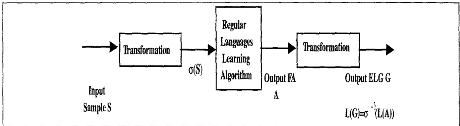
Figure 2: A scheme to learn Even Linear Languages.
